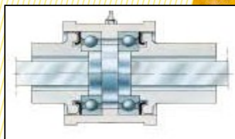
Knife axle bearing construction in models 3800-4600-6400
